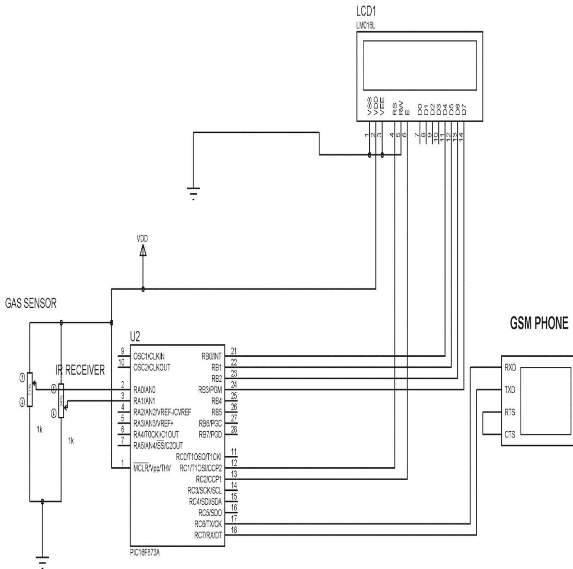
Fig1.0: Schematic diagram of home security simulation
